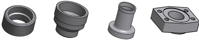
Threaded connection Victaulic connection Solder connection Flange Connection
